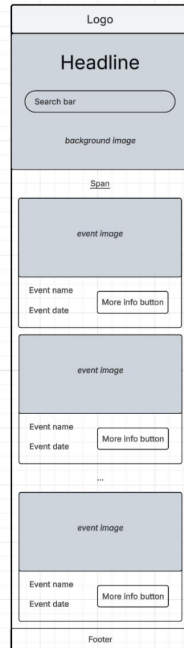
Landing page
